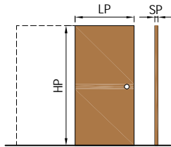
PANNELLO PORTA / PANEL PUERTA DOOR PANEL / PANNEAU PORTE
